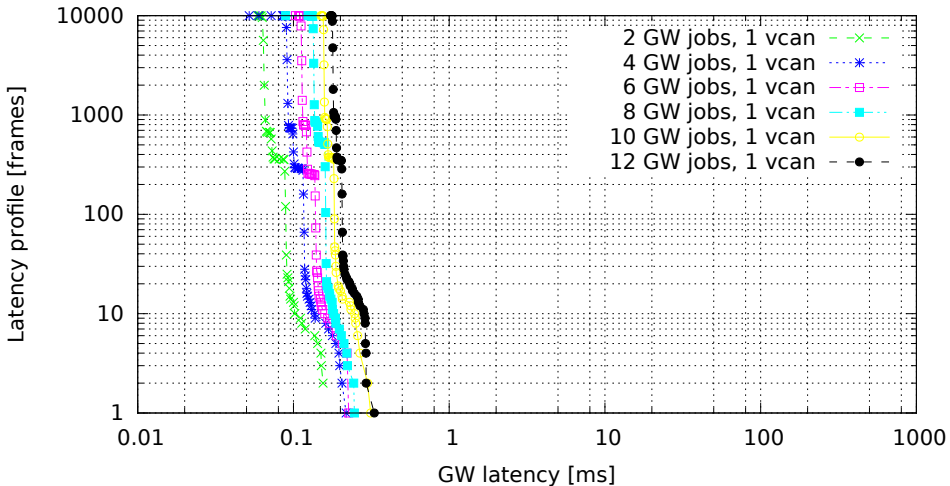
Chained GWs on a single VCAN interface (GW kernel 2.6.33.7-00007-g9c0ff90, Traffic oneatatime, Load none)
