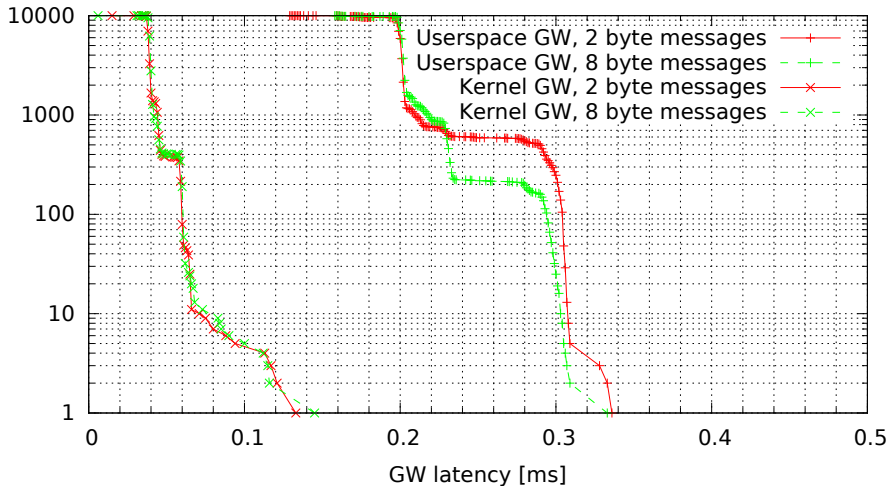
Kernel vs. userspace GW, no modifications (GW kernel 2.6.33.7-00007-g9c0ff90, Traffic oneatatime, Load none)
