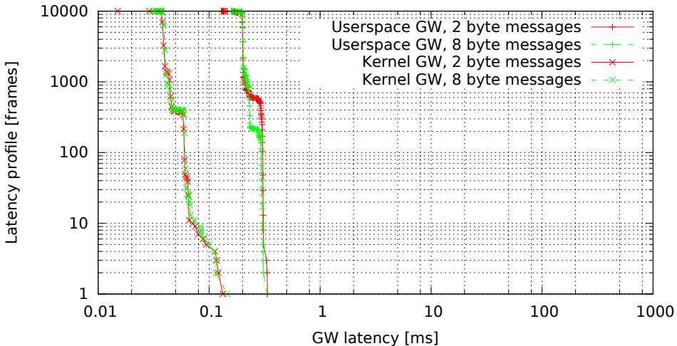
Kernel vs. userspace GW, no modifications (GW kernel 2.6.33.7-00007-g9c0ff90, Traffic oneatatime, Load none)
