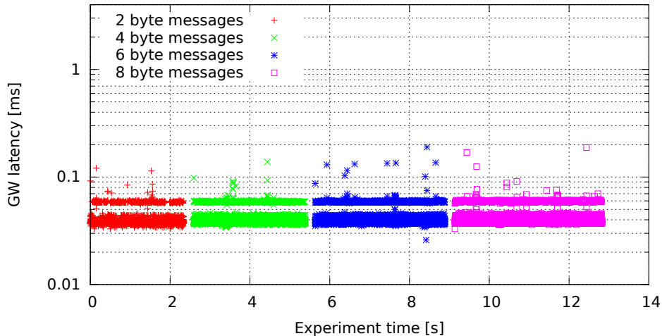
Single GW rule for all messages, no modifications (GW kernel 2.6.33.7-00007-g9c0ff90, Traffic oneatatime, Load none)
