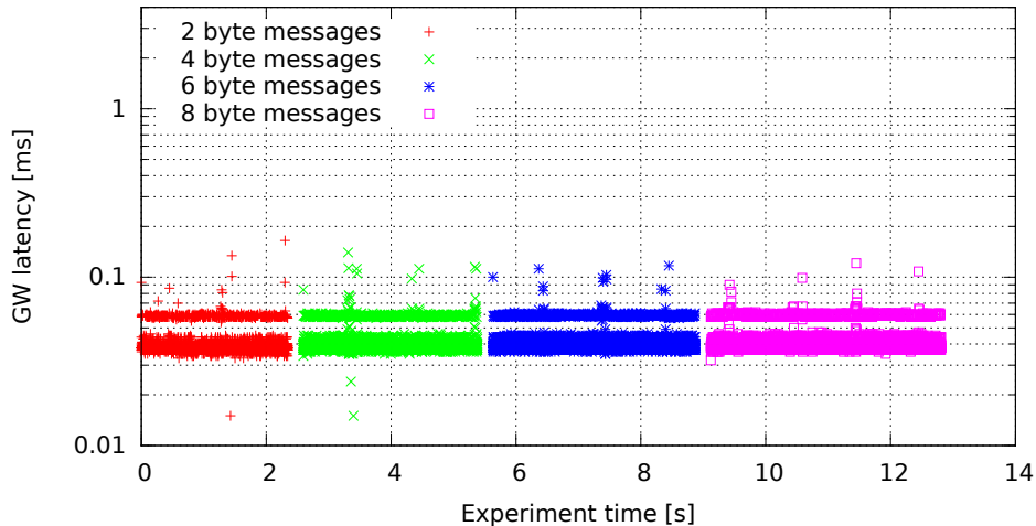
Single GW rule for all messages, no modifications, high (soft)irq task priority (GW kernel 2.6.33.7-00007-g9c0ff90, Traffic oneatatime, Load none)
