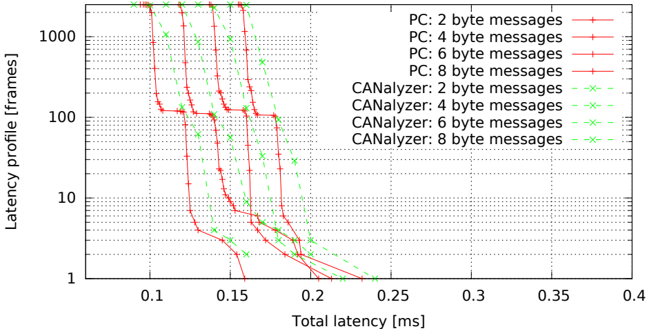
Measurement precision: PC versus CANalyzer (GW kernel 2.6.33.7-00007-g9c0ff90, Traffic oneatatime, Load none)
