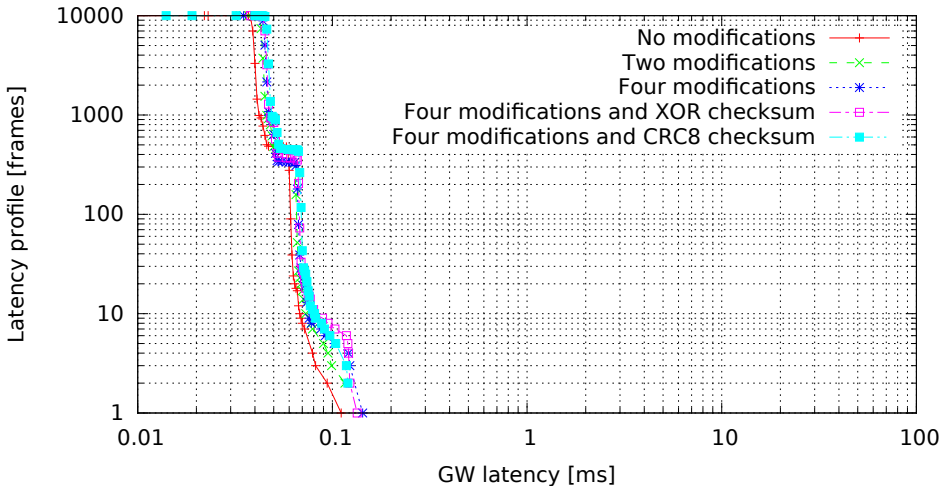
Single GW rule for all messages with modifications, 8 byte messages (GW kernel 2.6.33.7-00007-g9c0ff90, Traffic oneatatime, Load none)
