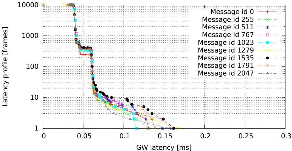
2048 GW rules (one per id, mask C00007FF), no modifications (GW kernel 2.6.33.7-00007-g9c0ff90, Traffic oneatatime, Load none)
