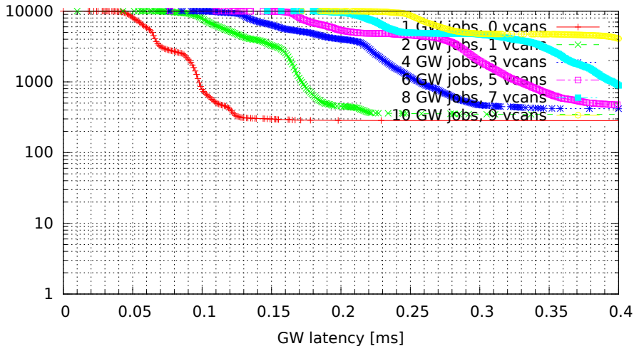
Chained GWs on multiple VCAN interfaces (GW kernel 2.6.33.7-00007-g9c0ff90, Traffic oneatatime, Load eth)
