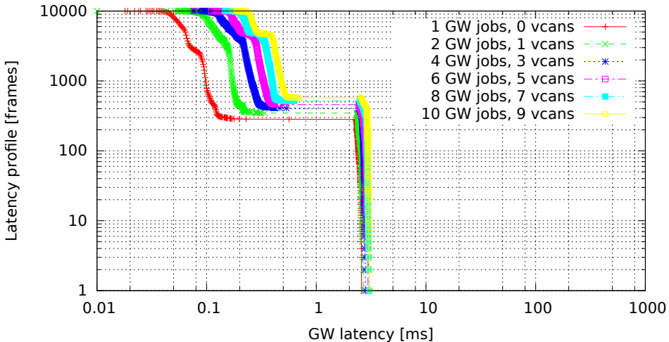
Chained GWs on multiple VCAN interfaces (GW kernel 2.6.33.7-00007-g9c0ff90, Traffic oneatatime, Load eth)
