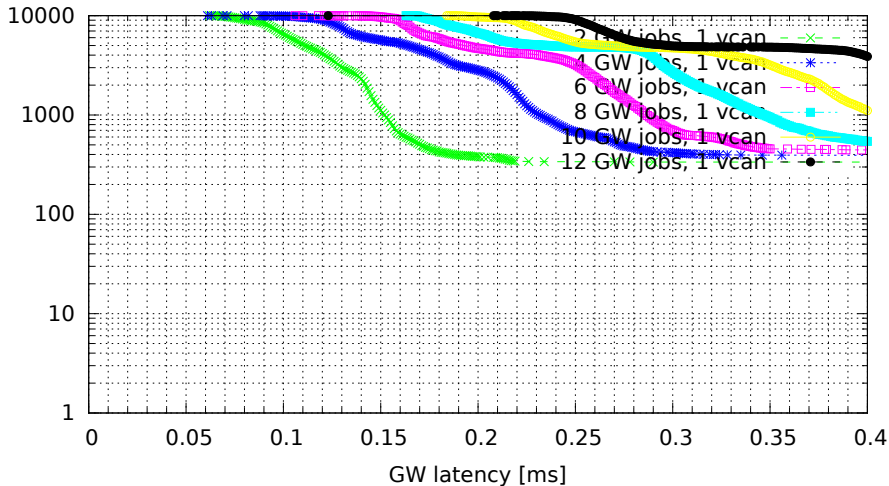
Chained GWs on a single VCAN interface (GW kernel 2.6.33.7-00007-g9c0ff90, Traffic oneatatime, Load eth)
