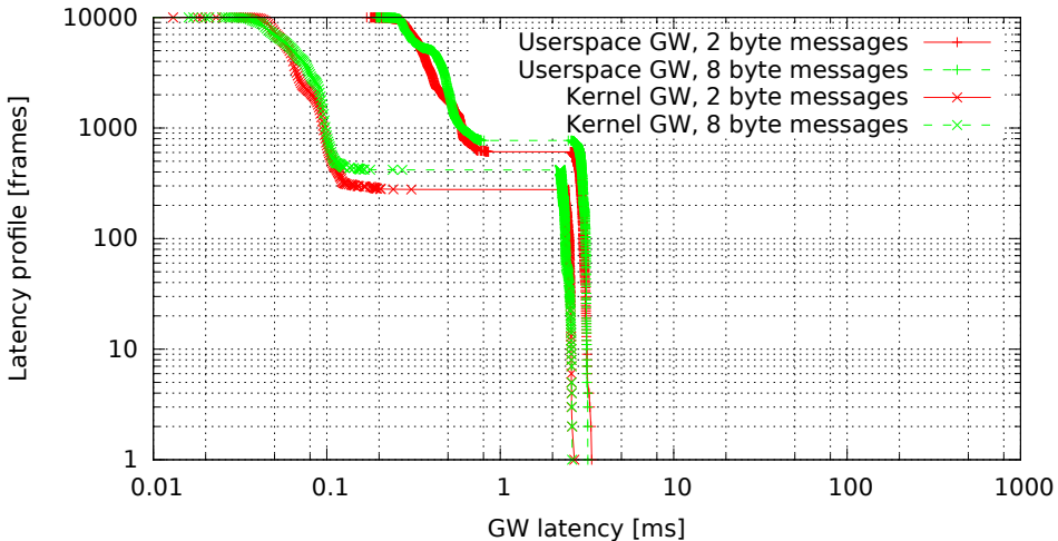
Kernel vs. userspace GW, no modifications (GW kernel 2.6.33.7-00007-g9c0ff90, Traffic oneatatime, Load eth)
