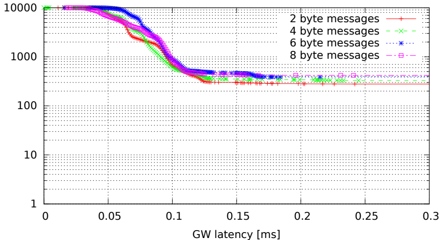
Single GW rule for all messages, no modifications (GW kernel 2.6.33.7-00007-g9c0ff90, Traffic oneatatime, Load eth)
