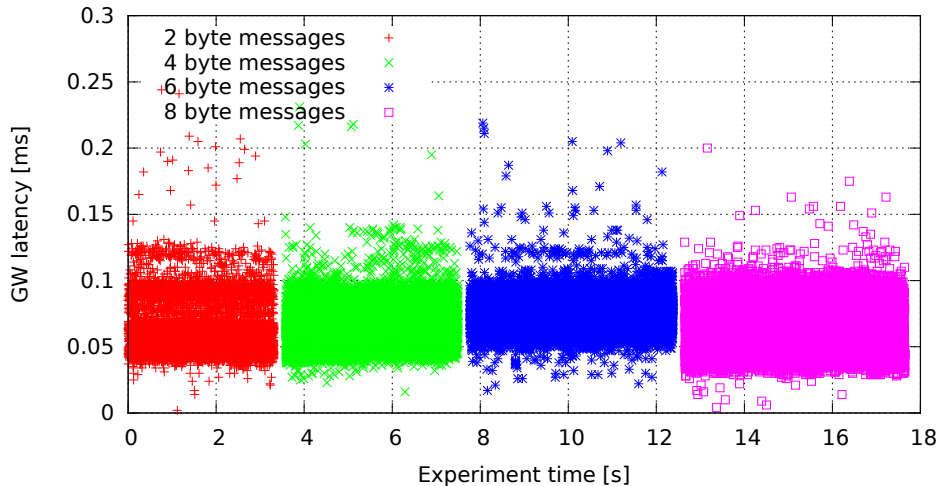
Single GW rule for all messages, no modifications, high (soft)irq task priority (GW kernel 2.6.33.7-00007-g9c0ff90, Traffic oneatatime, Load eth)
