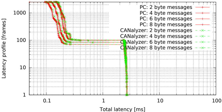
Measurement precision: PC versus CANalyzer (GW kernel 2.6.33.7-00007-g9c0ff90, Traffic oneatatime, Load eth)
