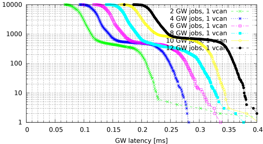
Chained GWs on a single VCAN interface (GW kernel 2.6.33.7-00007-g9c0ff90, Traffic oneatatime, Load cpu)
