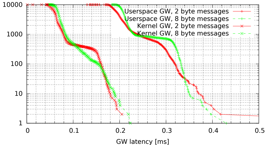
Kernel vs. userspace GW, no modifications (GW kernel 2.6.33.7-00007-g9c0ff90, Traffic oneatatime, Load cpu)
