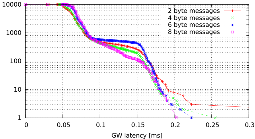
Single GW rule for all messages, no modifications (GW kernel 2.6.33.7-00007-g9c0ff90, Traffic oneatatime, Load cpu)
