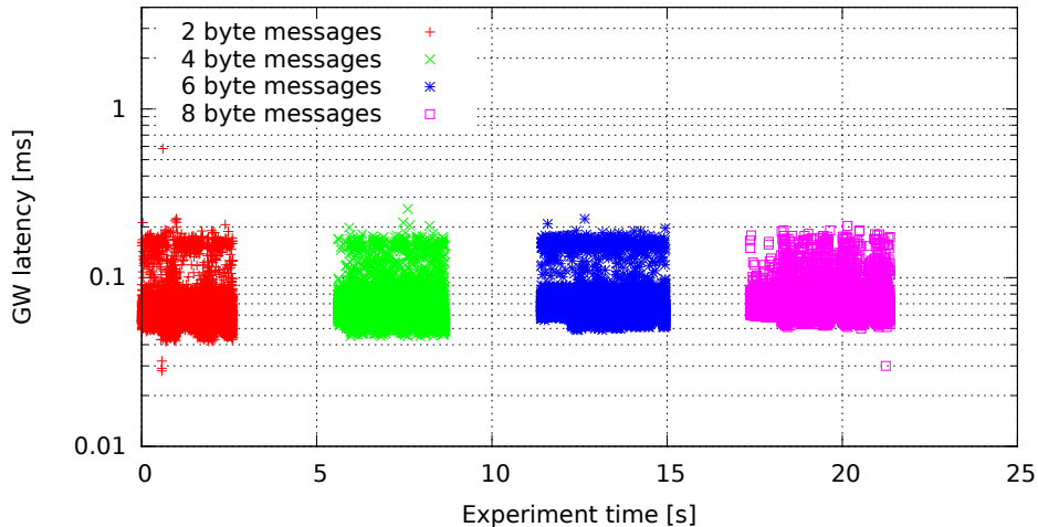
Single GW rule for all messages, no modifications (GW kernel 2.6.33.7-00007-g9c0ff90, Traffic oneatatime, Load cpu)
