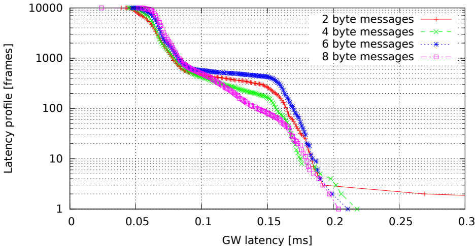
Single GW rule for all messages, no modifications, high (soft)irq task priority (GW kernel 2.6.33.7-00007-g9c0ff90, Traffic oneatatime, Load cpu)
