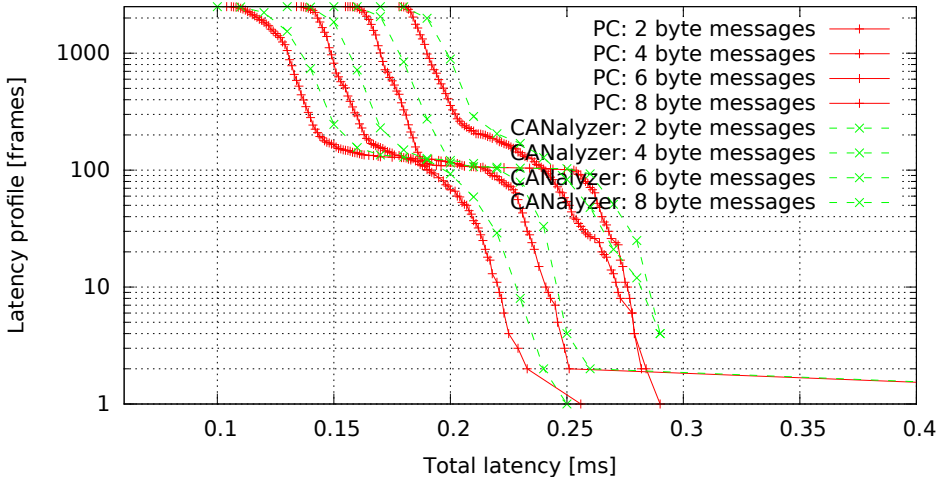
Measurement precision: PC versus CANalyzer (GW kernel 2.6.33.7-00007-g9c0ff90, Traffic oneatatime, Load cpu)
