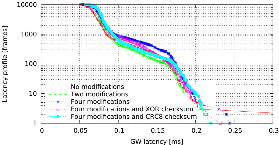
Single GW rule for all messages with modifications, 8 byte messages (GW kernel 2.6.33.7-00007-g9c0ff90, Traffic oneatatime, Load cpu)
