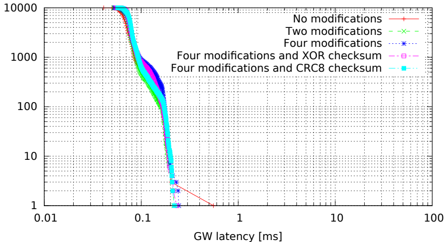
Single GW rule for all messages with modifications, 8 byte messages (GW kernel 2.6.33.7-00007-g9c0ff90, Traffic oneatatime, Load cpu)
