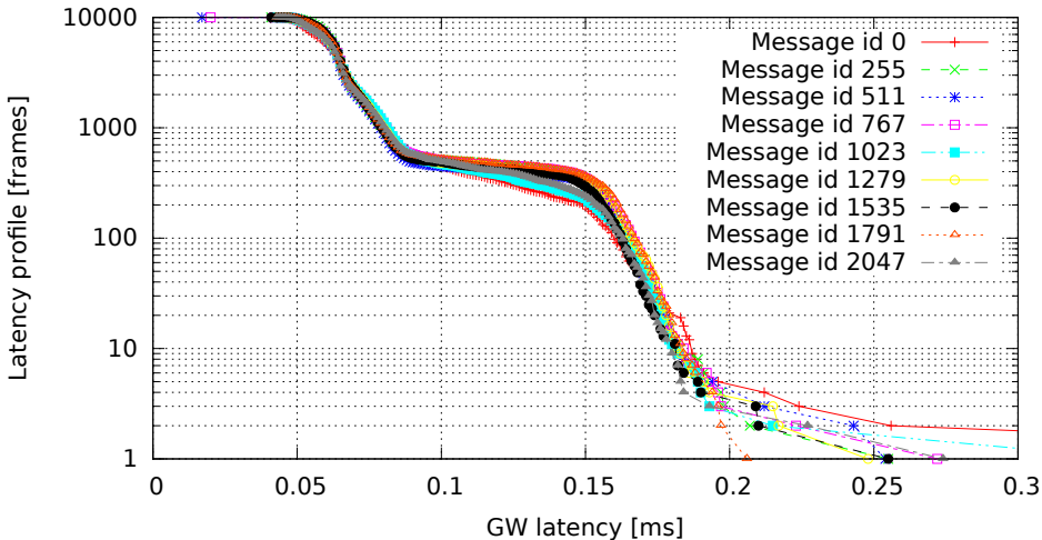
2048 GW rules (one per id, mask C00007FF), no modifications (GW kernel 2.6.33.7-00007-g9c0ff90, Traffic oneatatime, Load cpu)
