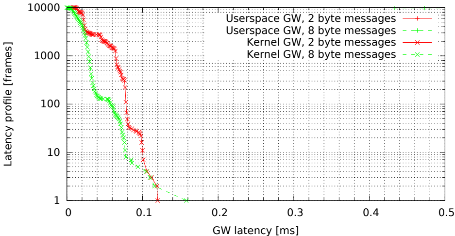
Kernel vs. userspace GW, no modifications (GW kernel 2.6.33.7-00007-g9c0ff90, Traffic flood, Load none)
