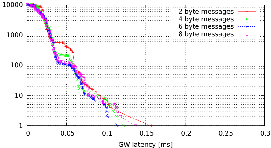
Single GW rule for all messages, no modifications (GW kernel 2.6.33.7-00007-g9c0ff90, Traffic flood, Load none)
