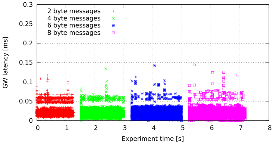
Single GW rule for all messages, no modifications, high (soft)irq task priority (GW kernel 2.6.33.7-00007-g9c0ff90, Traffic flood, Load none)
