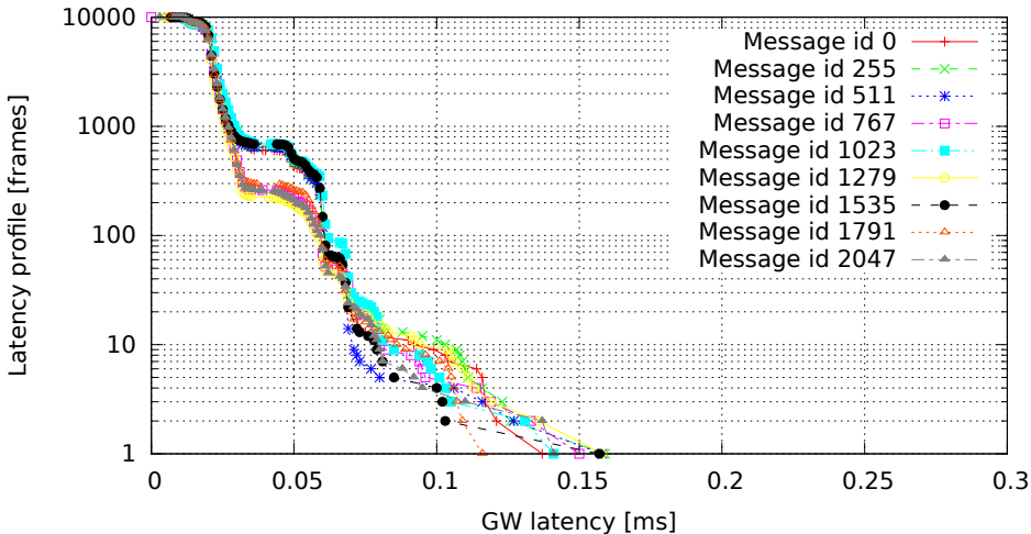
2048 GW rules (one per id, mask C00007FF), no modifications (GW kernel 2.6.33.7-00007-g9c0ff90, Traffic flood, Load none)
