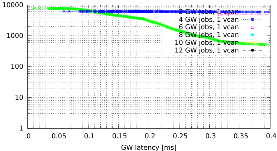
Chained GWs on a single VCAN interface (GW kernel 2.6.33.7-00007-g9c0ff90, Traffic flood, Load eth)
