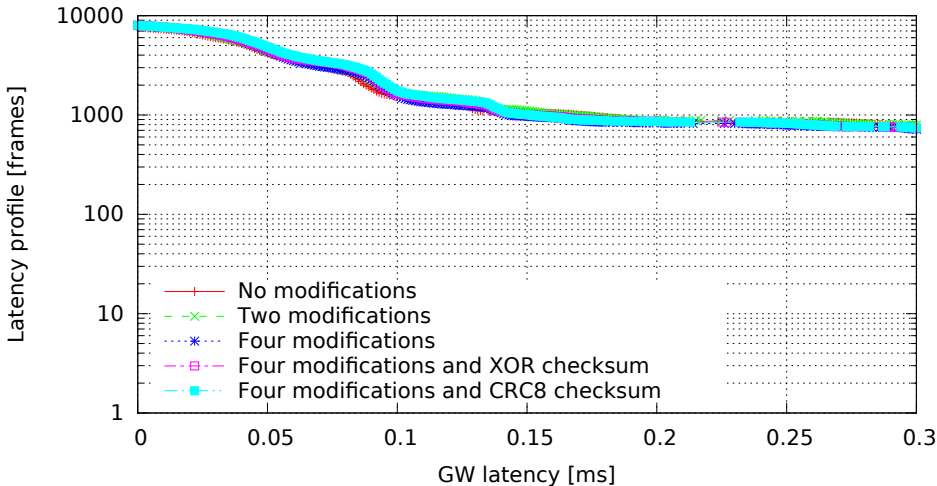
Single GW rule for all messages with modifications, 8 byte messages (GW kernel 2.6.33.7-00007-g9c0ff90, Traffic flood, Load eth)
