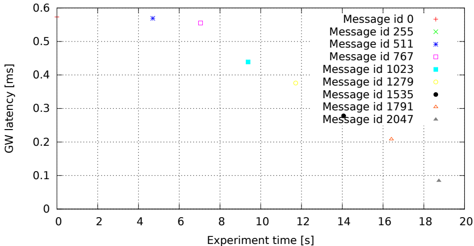
2048 GW rules (one per id, mask 0x7FF), no modifications (GW kernel 2.6.33.7-00007-g9c0ff90, Traffic flood, Load eth)
