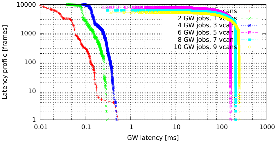
Chained GWs on multiple VCAN interfaces (GW kernel 2.6.33.7-00007-g9c0ff90, Traffic flood, Load cpu)
