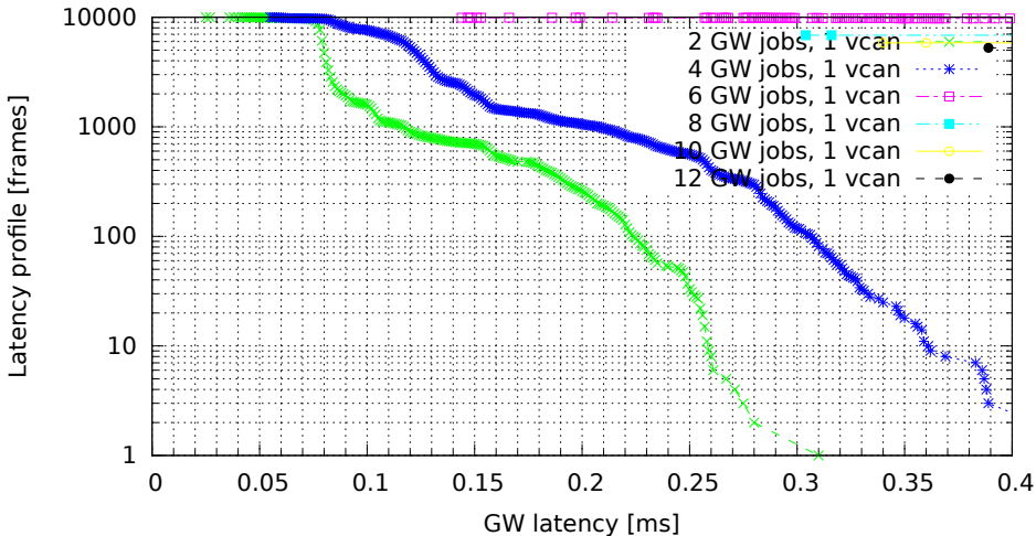
Chained GWs on a single VCAN interface (GW kernel 2.6.33.7-00007-g9c0ff90, Traffic flood, Load cpu)
