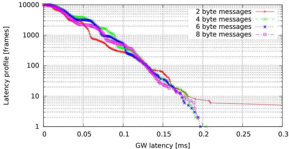
Single GW rule for all messages, no modifications (GW kernel 2.6.33.7-00007-g9c0ff90, Traffic flood, Load cpu)
