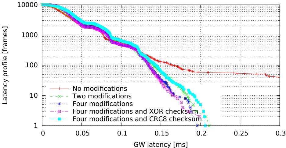
Single GW rule for all messages with modifications, 8 byte messages (GW kernel 2.6.33.7-00007-g9c0ff90, Traffic flood, Load cpu)
