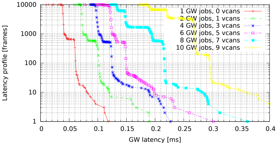
Chained GWs on multiple VCAN interfaces (GW kernel 2.6.33.7-00007-g9c0ff90, Traffic 50, Load none)
