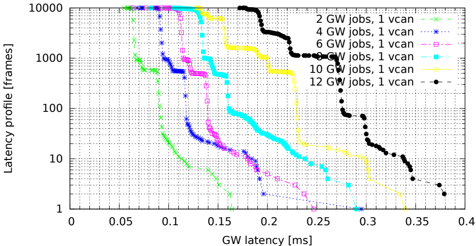
Chained GWs on a single VCAN interface (GW kernel 2.6.33.7-00007-g9c0ff90, Traffic 50, Load none)
