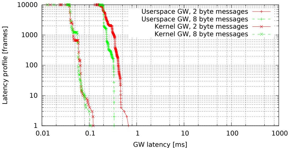
Kernel vs. userspace GW, no modifications (GW kernel 2.6.33.7-00007-g9c0ff90, Traffic 50, Load none)
