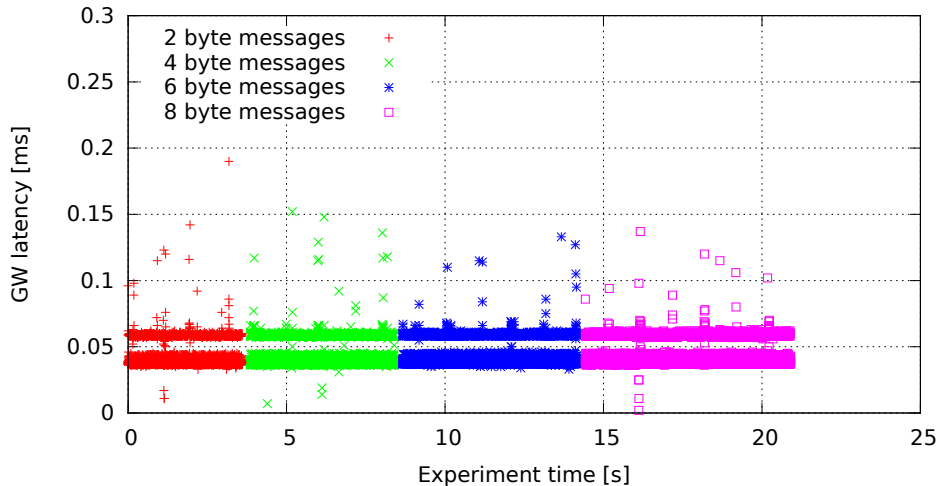
Single GW rule for all messages, no modifications (GW kernel 2.6.33.7-00007-g9c0ff90, Traffic 50, Load none)
