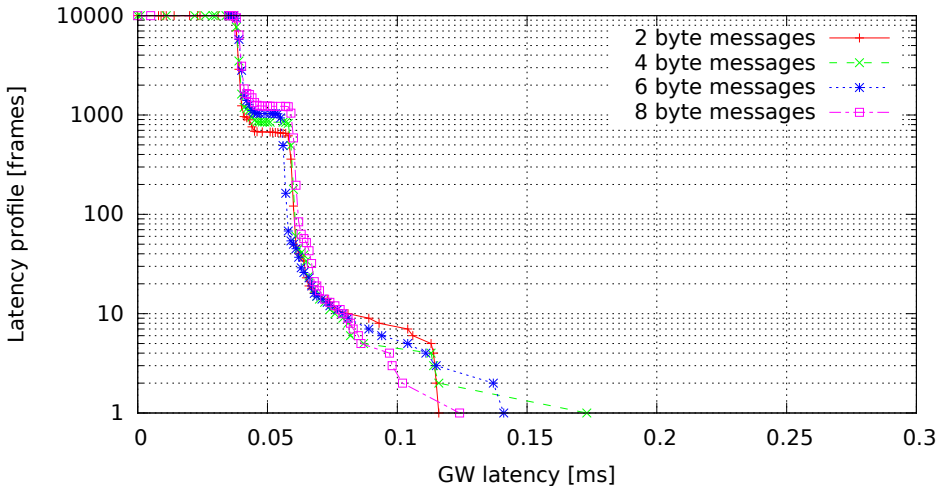
Single GW rule for all messages, no modifications, high (soft)irq task priority (GW kernel 2.6.33.7-00007-g9c0ff90, Traffic 50, Load none)
