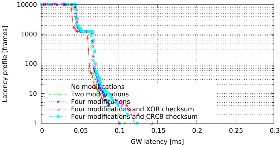
Single GW rule for all messages with modifications, 8 byte messages (GW kernel 2.6.33.7-00007-g9c0ff90, Traffic 50, Load none)
