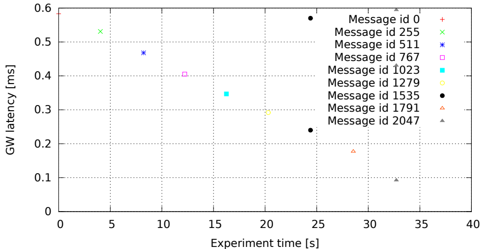
2048 GW rules (one per id, mask 0x7FF), no modifications (GW kernel 2.6.33.7-00007-g9c0ff90, Traffic 50, Load none)
