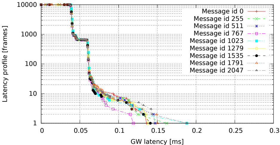
2048 GW rules (one per id, mask C00007FF), no modifications (GW kernel 2.6.33.7-00007-g9c0ff90, Traffic 50, Load none)
