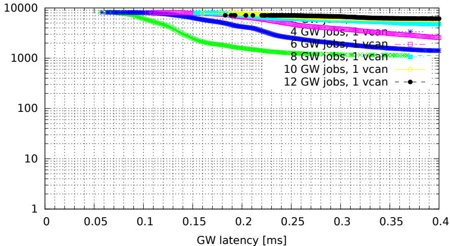
Chained GWs on a single VCAN interface (GW kernel 2.6.33.7-00007-g9c0ff90, Traffic 50, Load eth)
