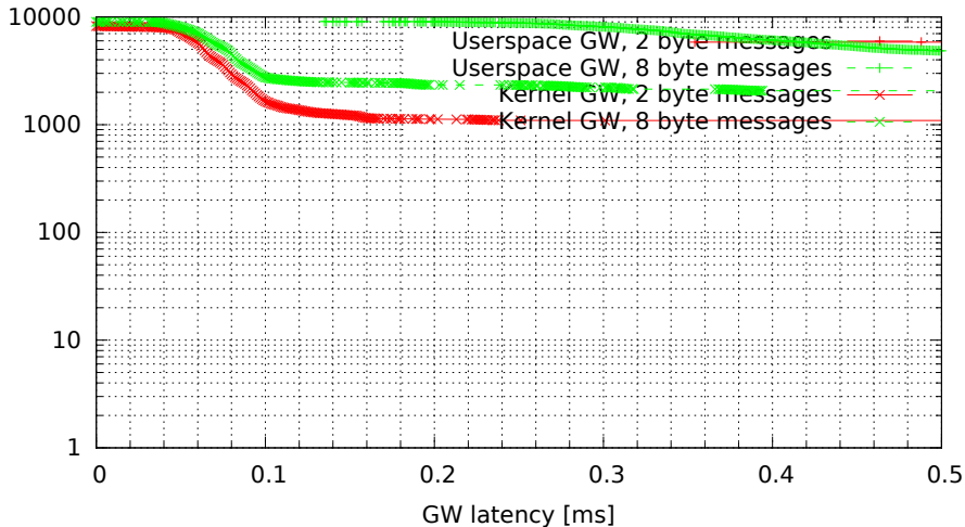
Kernel vs. userspace GW, no modifications (GW kernel 2.6.33.7-00007-g9c0ff90, Traffic 50, Load eth)
