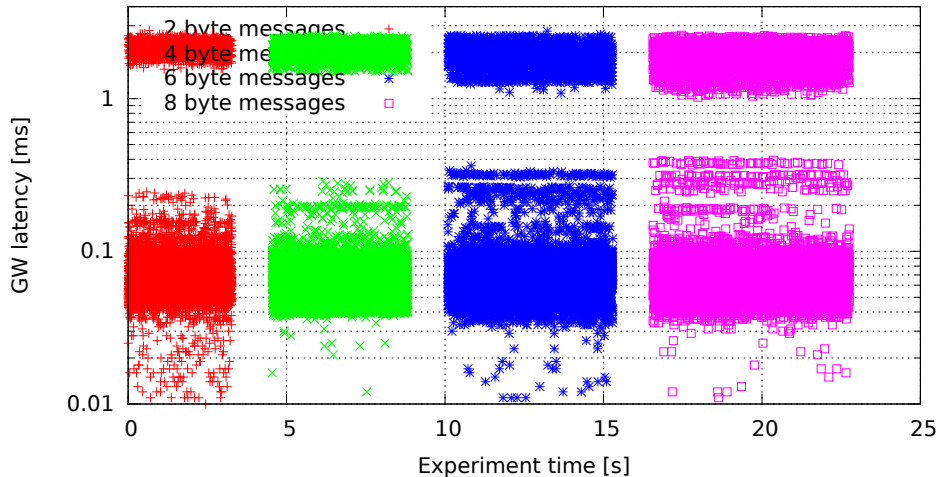
Single GW rule for all messages, no modifications (GW kernel 2.6.33.7-00007-g9c0ff90, Traffic 50, Load eth)
