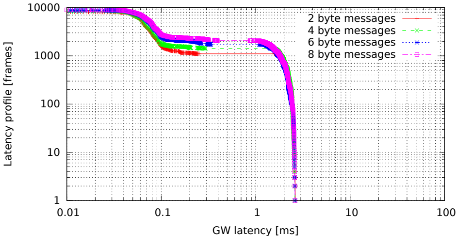
Single GW rule for all messages, no modifications, high (soft)irq task priority (GW kernel 2.6.33.7-00007-g9c0ff90, Traffic 50, Load eth)
