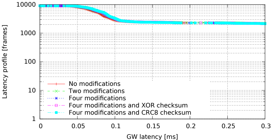
Single GW rule for all messages with modifications, 8 byte messages (GW kernel 2.6.33.7-00007-g9c0ff90, Traffic 50, Load eth)
