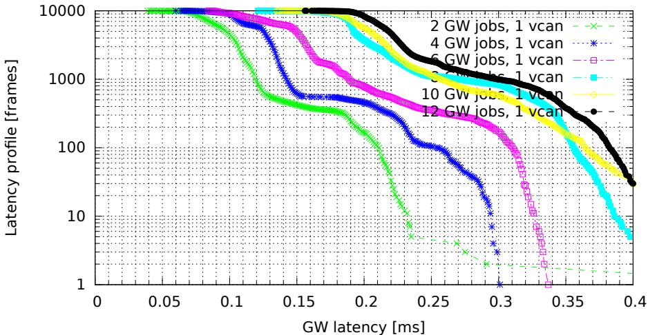
Chained GWs on a single VCAN interface (GW kernel 2.6.33.7-00007-g9c0ff90, Traffic 50, Load cpu)
