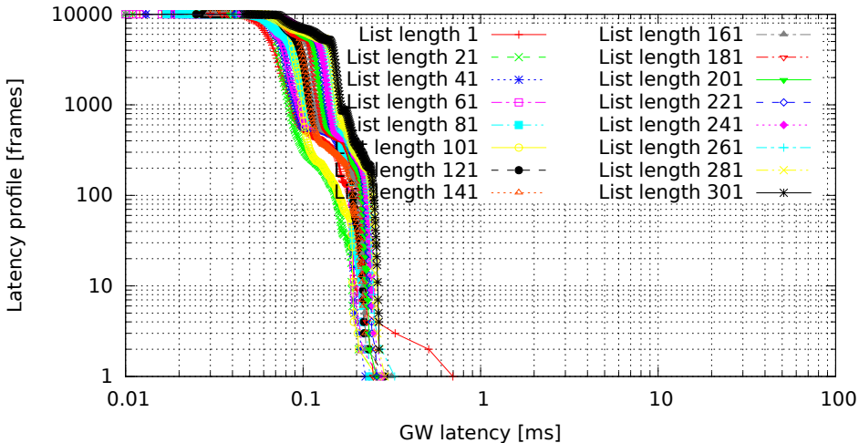
Different lengths of filter list, only the last one matches (GW kernel 2.6.33.7-00007-g9c0ff90, Traffic 50, Load cpu)
